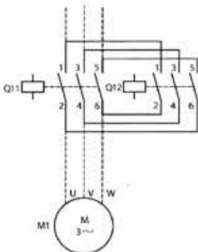
Reversing contactors
