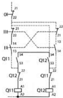
Reversing contactors
