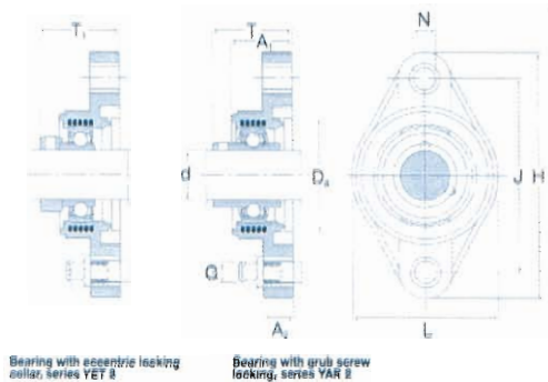
Bearing with eccentric locking collar, series YET 2
